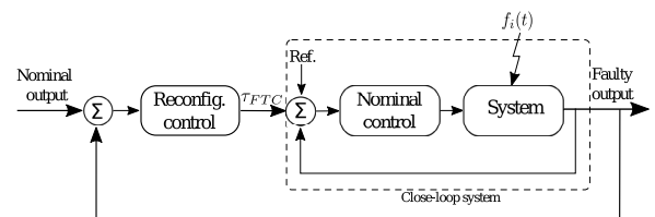
Fig. 2. Structure to get recoverable faults.
