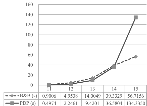
Fig. 4. Execution time of B&B and PDP with respect to n when m = 4 .
