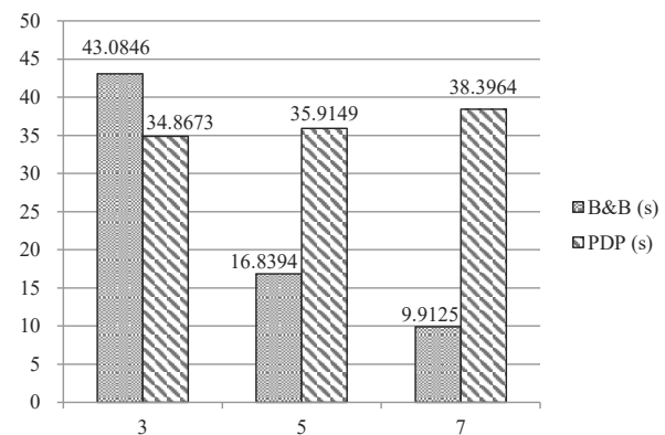
Fig. 5. Execution time of B&B and PDP with respect to \beta .
