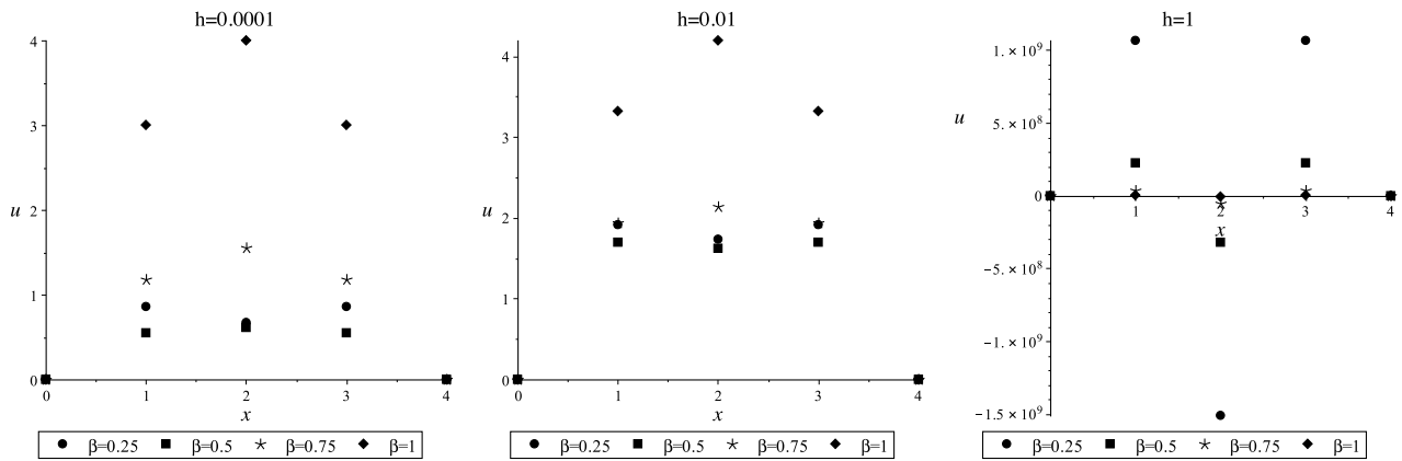
Fig. 4. Diffusion concentration versus the discrete space x for \beta = 0.25, 0.5, 0.75 , and h = 0.0001, 0.01, 1 (in the case of Eqn. (38)).
