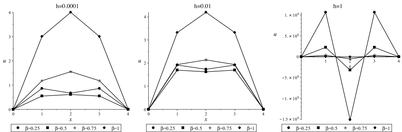
Fig. 5. Diffusion concentration versus the discrete space x for \beta = 0.25, 0.5, 0.75 , and h = 0.0001, 0.01, 1 (in the case of Eqn. (38)).
