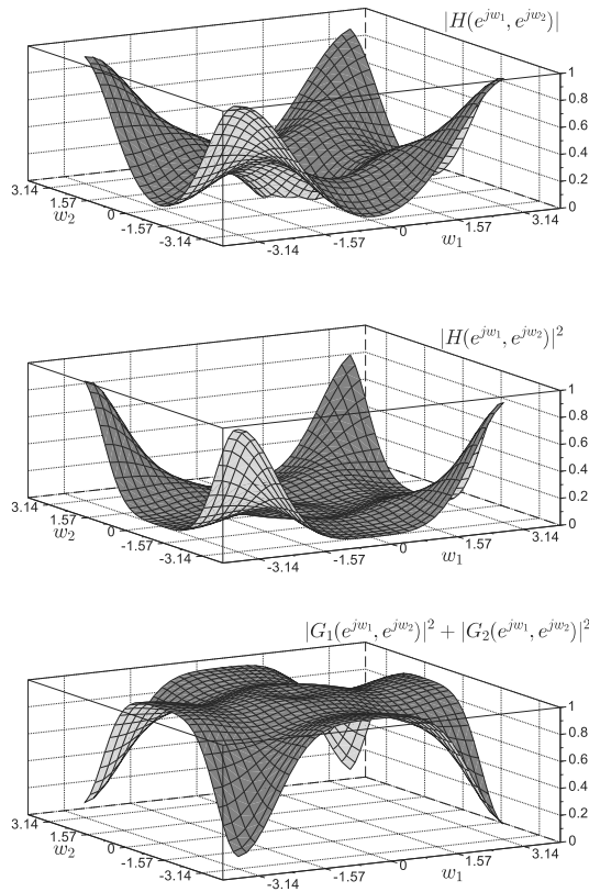
Fig. 2. High-pass sharpening filter with octagonal symmetry: amplitude characteristics of |H(e^{j\omega_1}, e^{j\omega_2})| , |H(e^{j\omega_1}, e^{j\omega_2})|^2 , |G_1(e^{j\omega_1}, e^{j\omega_2})|^2 + |G_2(e^{j\omega_1}, e^{j\omega_2})|^2 .
