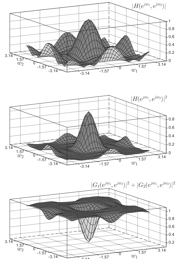
Fig. 9. Low-pass denoising filter from approximation with octagonal symmetry: amplitude characteristics of |H(e^{j\omega_1}, e^{j\omega_2})| , |H(e^{j\omega_1}, e^{j\omega_2})|^2 , and |G_1(e^{j\omega_1}, e^{j\omega_2})|^2 + |G_2(e^{j\omega_1}, e^{j\omega_2})|^2 .
