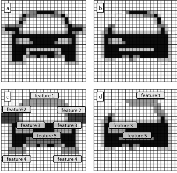
Fig. 3. Problem of classification based on the evaluation of features: original pattern (a), noisy pattern (b), decomposition of features of the original pattern (c), decomposition of features of the noisy pattern (d).
