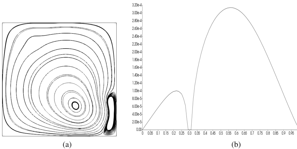
Fig. 3. Example 1: streamline for the Stokes–Darcy flow in \Omega_\rho with \gamma = 10^{10} (a), plot over the line y = 0.8 (b).
