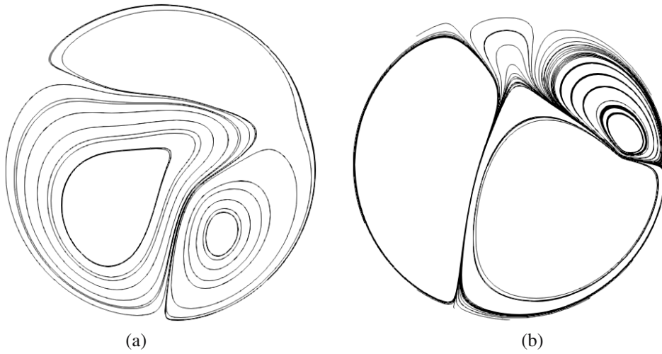
Fig. 7. Example 2: streamline for the controlled state y(\bar{u}, \bar{\tau}) (a), streamline for the adjoint state v (b).
